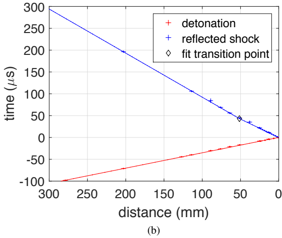
Fig. 13 x-t diagram showing detonation and shock arrivals for shots (a) 2163 and (b) 2180 with initial composition of stoichiometric hydrogen-oxygen at fill pressure 10 and 50 kPa respectively. The detonation is modeled with constant speed, U_{\text{det}} , and the reflected shock is modeled as having constant speeds U_{\text{RS,w}} for x < x_t and U_{\text{RS,}\infty} for x > x_t .
