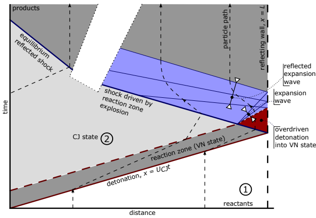
Fig. 17 Space-time diagram of the simplified reflecting detonation model with finite-length reaction zone. The transition region where the reflected expansion wave catches the reflected shock is condensed in the blank region of the schematic to allow greater detail of the reaction zone.
