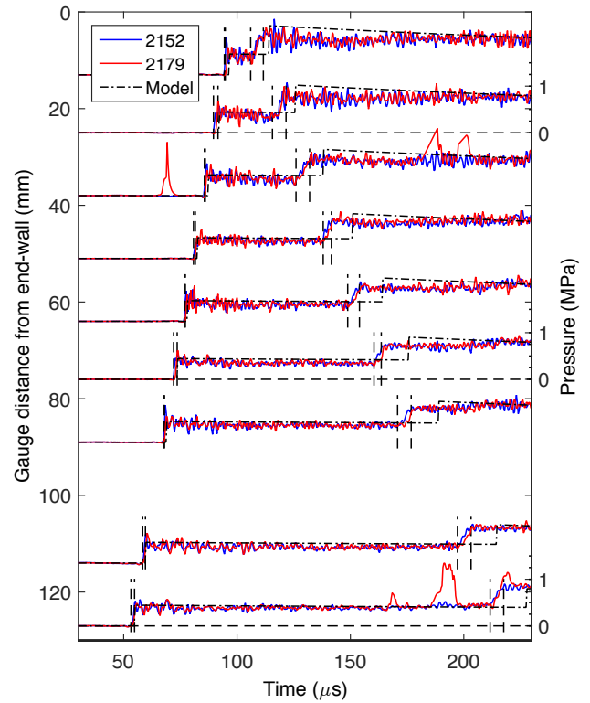
Fig. 15 Pressure measurements for shots 2152 and 2179 compared to a one-dimensional infinitesimal-length reaction zone pressure model that incorporates the TZ expansion. The initial composition was stoichiometric hydrogen-oxygen at fill pressure 25 kPa.
