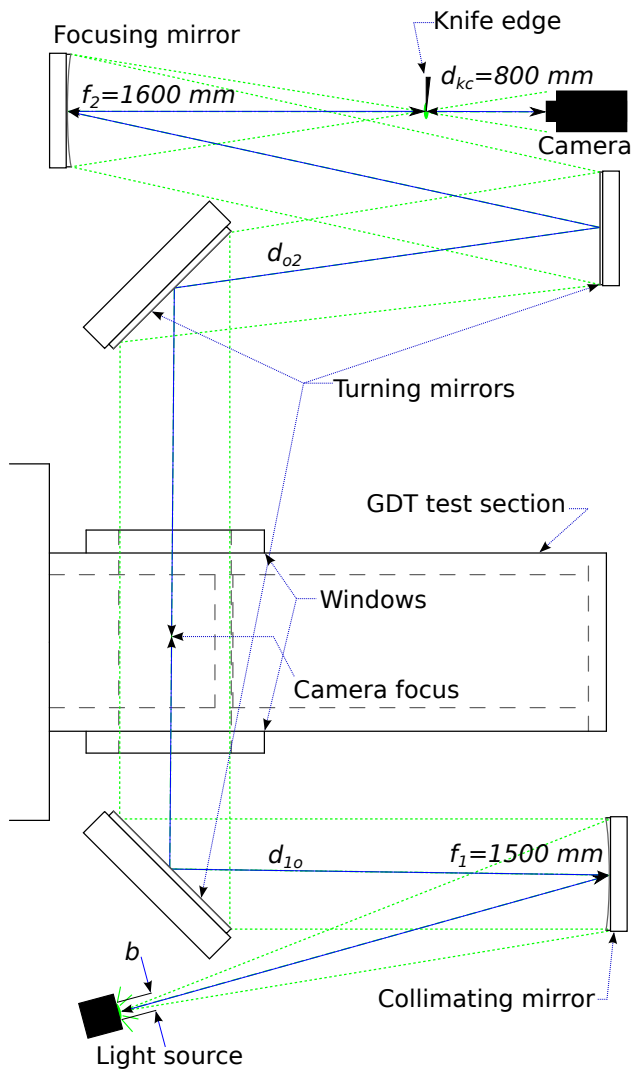
Fig. 3 Schematic of schlieren visualization system and GDT test section as viewed from above.
