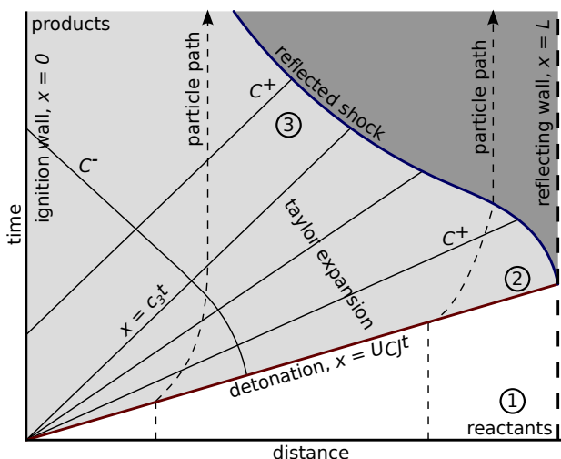
Fig. 1 Space-time diagram of a reflecting detonation and attached Taylor-Zel'dovich expansion wave. The detonation reflects off the wall located at x = L and the reflected shock wave passes through the expansion.
