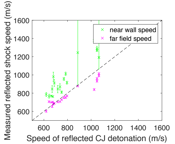
Fig. 14 Measured reflected shock speed at the wall U_{\text{RS,w}} , and in the far field U_{\text{RS,}\infty} , compared to the idealized reflected shock speed U_{\text{R,CJ}} . The dashed black line corresponds to U_{\text{measured}} = U_{\text{R,CJ}} .
