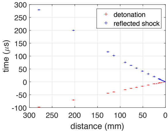
Fig. 6 x - t diagram showing detonation and shock arrivals, with uncertainties, for representative shot 2152. The detonation propagates towards the end-wall at the right, and the reflected shock propagates back. The points clustered near the end-wall correspond to arrivals taken from the image files, and the points farther away correspond to arrivals taken from the pressure measurements.
