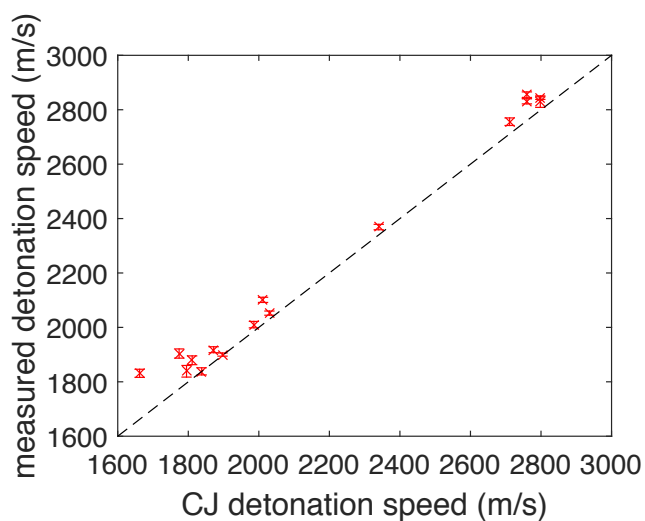
Fig. 11 Measured detonation speed compared to the theoretical CJ detonation speed. The dashed line corresponds to U_{\text{det}} = U_{\text{CJ}} .
