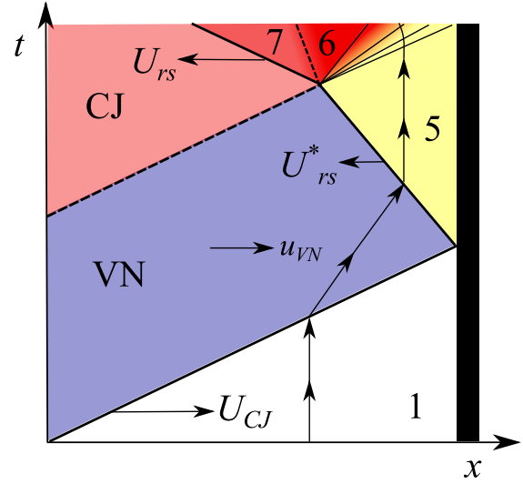
Fig. 18 Reflection of the leading shock wave into reaction zone of incident detonation.
