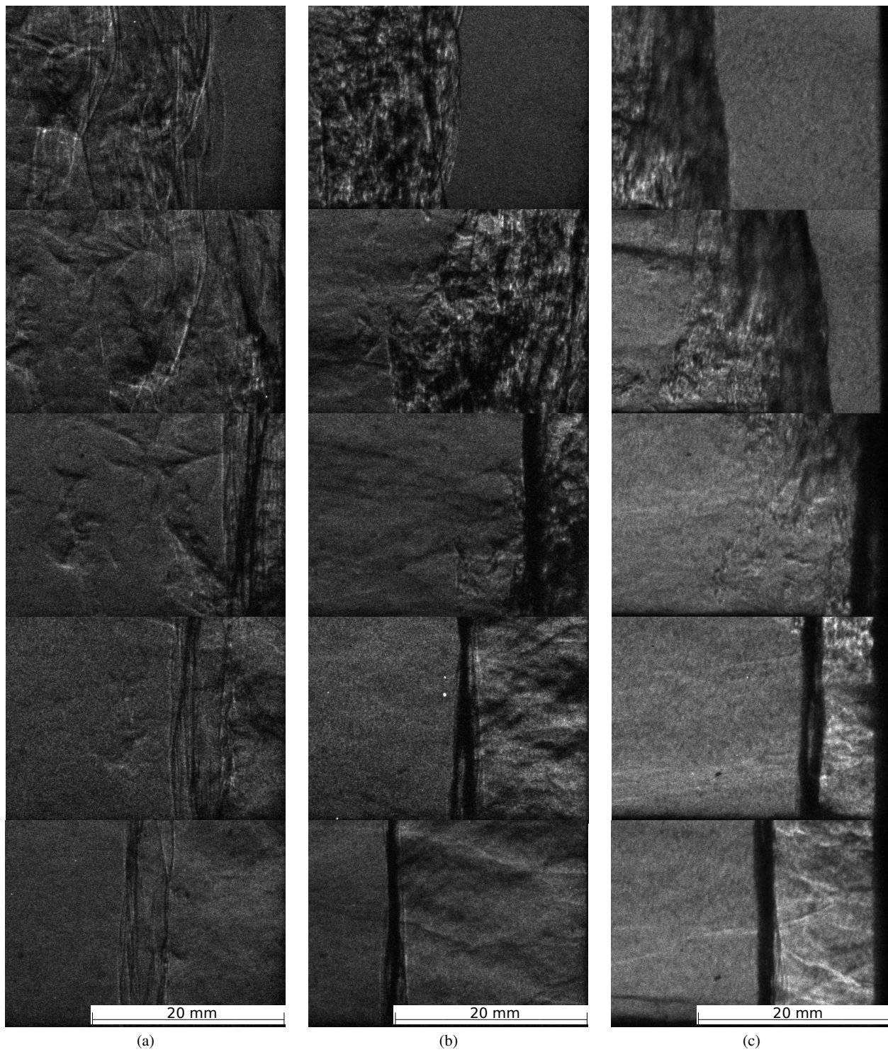
Fig. 8 Schlieren images of incident detonation and reflected shock wave for shots (a) 2168, (b) 2158, and (c) 2181. The initial mixture was stoichiometric hydrogen-oxygen with 33% carbon dioxide dilution at fill pressure 10, 25, and 50 kPa, respectively.
