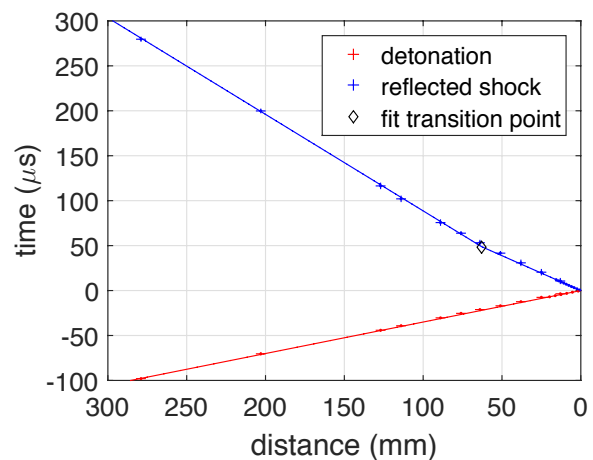
Fig. 12 x-t diagram showing detonation and shock arrivals for representative shot 2152 with initial composition of stoichiometric hydrogen-oxygen at fill pressure 25 kPa. The detonation is modeled with constant speed, U_{\text{det}} , and the reflected shock is modeled as having constant speeds U_{\text{rs,w}} for x < x_t and U_{\text{rs},\infty} for x > x_t .
