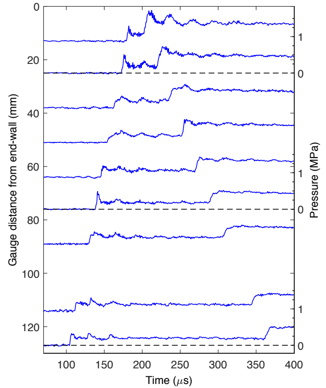
Fig. 10 Pressure measurements for shot 2166. The initial composition was stoichiometric hydrogen-oxygen with 80% argon dilution at fill pressure 10 kPa.
