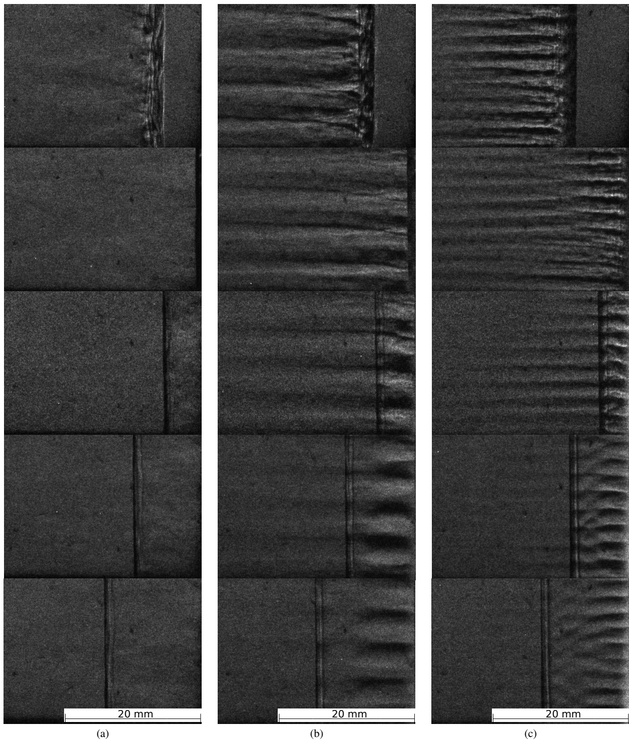
Fig. 7 Schlieren images of incident detonation and reflected shock wave for shots (a) 2164, (b) 2161, and (c) 2170. The initial mixture was stoichiometric hydrogen-oxygen with 50% argon dilution at fill pressure 10, 25, and 50 kPa, respectively.
