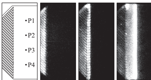
Figure 5. Static initiator results showing a schematic of the imaging area along with images taken 360 \mu\text{s} , 370 \mu\text{s} , and 375 \mu\text{s} after ignition. Each image was taken during a separate experiment. The test mixture was stoichiometric propane-oxygen at 1.0 bar.
