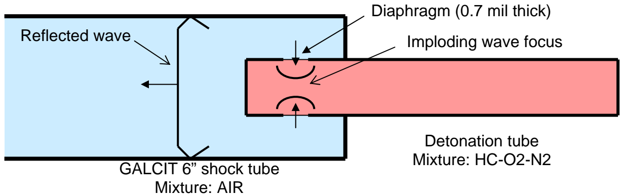
Figure 1. Schematic of annular jet imploding shock wave facility.
