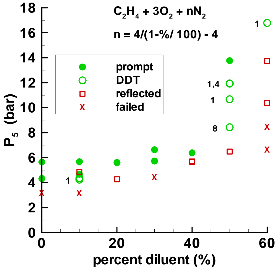
Figure 3. Experimental results for annular jet imploding shock initiator tests with stoichiometric ethylene-oxygen-nitrogen mixtures. The numbers indicate the ion probe location closest to the DDT event. Ion probe location 1 is closest to the annular orifice and location 9 is furthest from the orifice.
