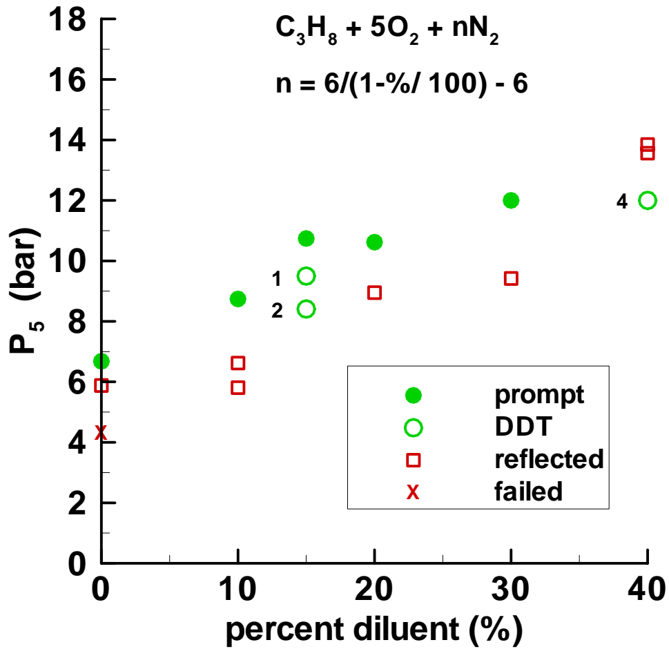
Figure 4. Experimental results for annular jet imploding shock initiator tests with stoichiometric propane-oxygen-nitrogen mixtures. The numbers indicate the ion probe location closest to the DDT event. Ion probe location 1 is closest to the annular orifice and location 9 is furthest from the orifice.
