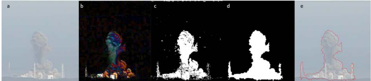
Figure 2: Image processing methodology to extract the contour of the debris plume - a) raw image, b) background removed, c) binarization by luminosity threshold, d) morphological operation, e) contour applied on the raw image
