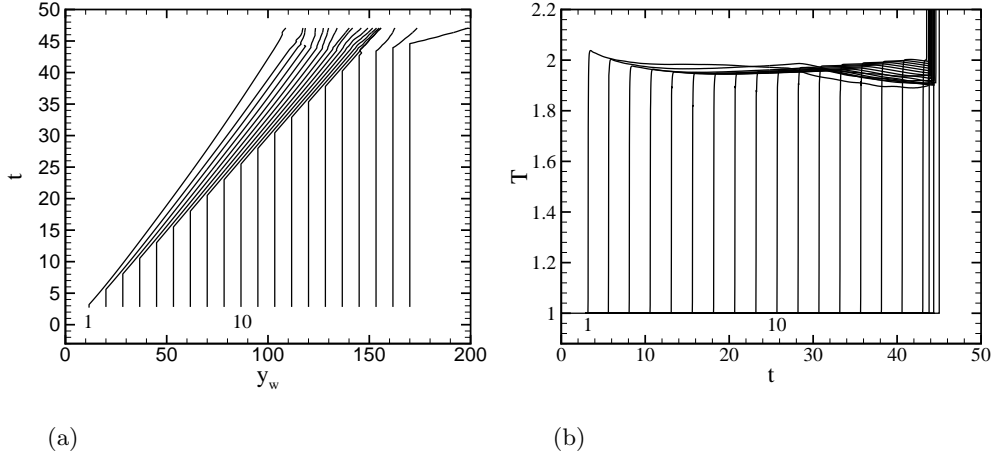
FIGURE 19. Frame (a): particle paths for 20 sample particles injected along the vertical corner wall (figure 9 (a)) for \theta_{CJ} = 3.5 . The labels 1 and 10 indicate the particles that are analyzed in terms of numerical dominant balance. Frame (b): temperature profiles along particles paths displayed in figure 19.
