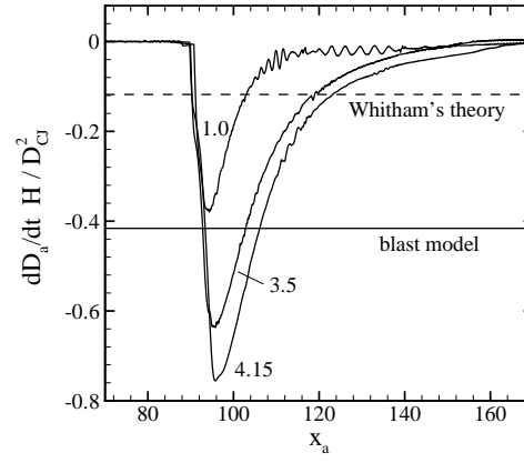
FIGURE 21. Shock deceleration as a function of the distance from the corner vertex, parametrized by \theta_{CJ} .
