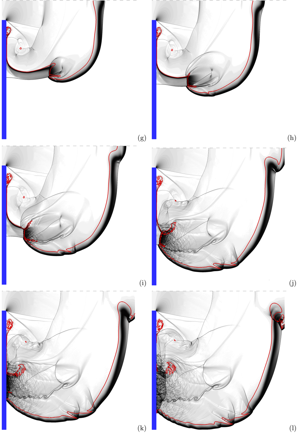
FIGURE 16. Numerical schlieren images for the case \theta_{CJ} = 3.5 . (g) t = 32.13 ; (h) t = 35.79 ; (i) t = 39.45 ; (j) t = 43.11 . (k) t = 44.94 ; (l) t = 46.77 .
