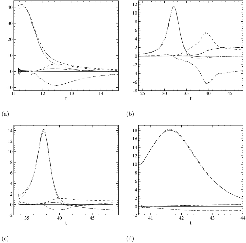
FIGURE 20. Terms in the reaction zone temperature (2.13) along the same particle paths as in figure 18 (a) for the case \theta_{CJ} = 3.5 . The particles are injected along the plane of symmetry. \cdots Lagrangian temperature; -\cdot-\cdot heat release; --- curvature; — transverse divergence; -\cdot-\cdot- unsteadiness. The solid line is the difference between the left-hand side and the right-hand side in (2.13), as computed from the terms above. (a) Particle 1; (b) Particle 10.; (c) Particle 16; (d) Particle 21.
