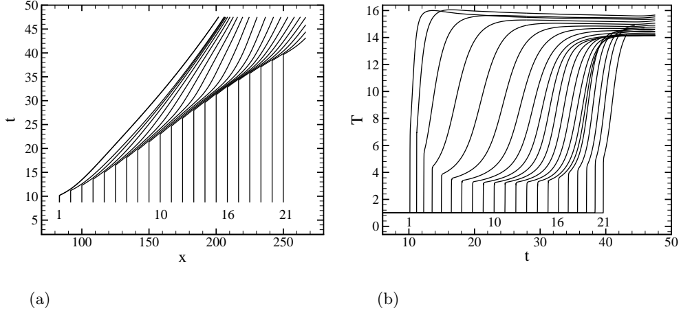
FIGURE 18. Frame (a): particle paths for 21 sample particles injected along the channel plane of symmetry (figure 9 (b)) for \theta_{CJ} = 3.5 . The labels 1, 10, 16, 21 indicate particles that are analyzed in terms of numerical dominant balance. Frame (b): temperature profiles along the particle paths.
