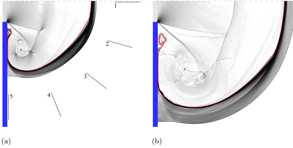
FIGURE 11. Numerical schlieren images for the case \theta_{CJ} = 4.15 at (a) t = 28.43 ; (b) t = 53.22 .
