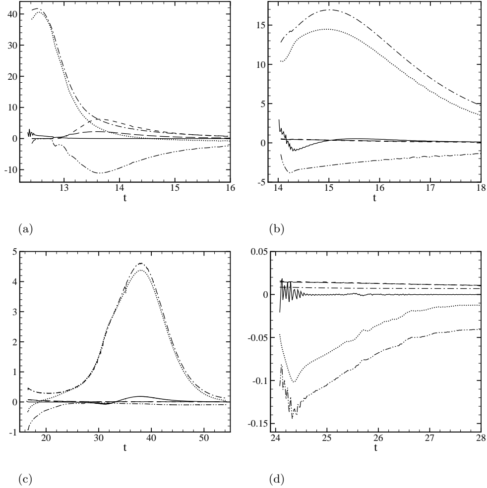
FIGURE 14. Terms in the reaction zone temperature (2.13) along the same particle paths as in figure 13 for \theta_{CJ} = 4.15 . The particles are injected on the channel plane of symmetry. \cdots Lagrangian temperature; -\cdot-\cdot heat release; --- curvature; --- transverse divergence; -\cdot-\cdot unsteadiness. The solid line is the difference between the left-hand side and the right-hand side in (2.13), as computed from the terms above. (a) Particle 1; (b) Particle 3; (c) Particle 5; (d) Particle 10.
