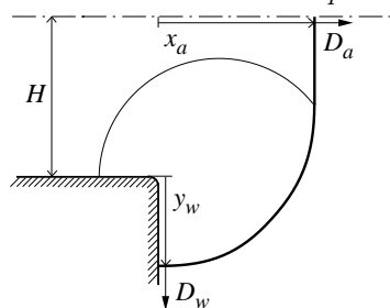
FIGURE 2. Detonation diffraction around a corner. -\cdot-\cdot- denotes the plane of symmetry of the channel, H the channel half-width. Also shown are the distances measured along the plane of symmetry, x_a , and along the corner wall, y_w .
