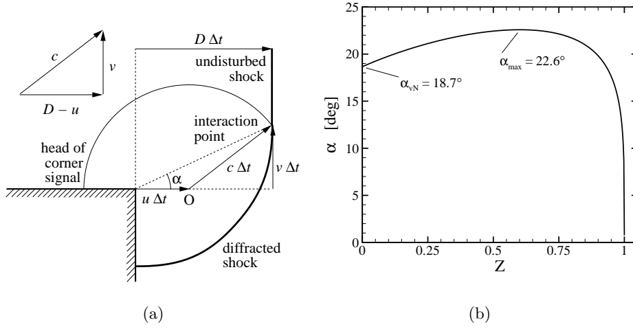
FIGURE 1. (a) Schematic of a diffracting shock (Skews' construction) in nonreactive gas. (b) Disturbance angle plotted vs. progress variable Z for a ZND-CJ detonation. Z = 0 corresponds to post-shock conditions, Z = 1 corresponds to the end of the reaction zone.
