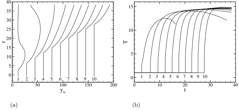
FIGURE 10. Frame(a): particle paths for 10 sample particles injected along the vertical corner wall for \theta_{CJ} = 1 . Frame (b): temperature profiles along the particle paths.
