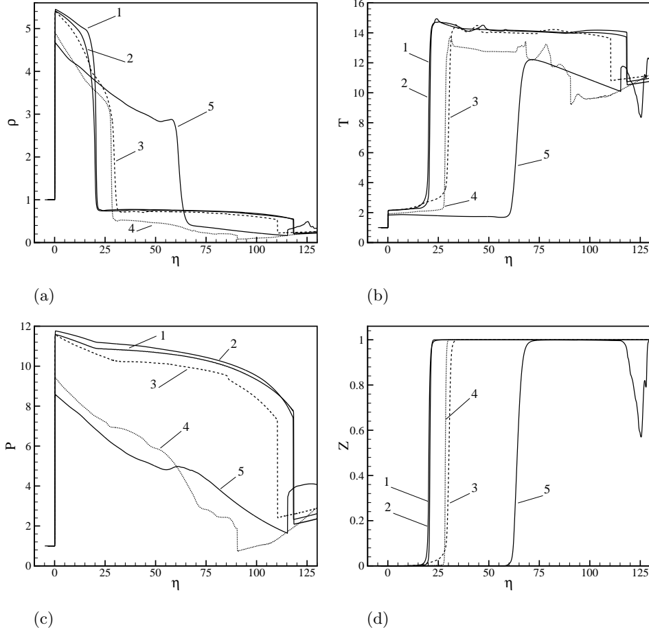
FIGURE 12. Density (a), temperature (b), pressure (c) and progress variable (d) profiles for 5 data sets extracted at t = 53.22 .
