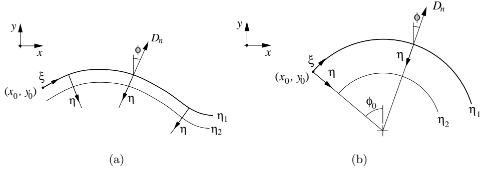
FIGURE 3. Intrinsic coordinates \xi and \eta for an arbitrary front, (a), and specialized to a cylindrical front, (b).
