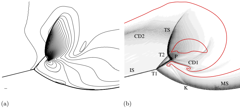
FIGURE 17. Structure of the re-ignition transverse wave: contours of pressure, (a), and numerical schlieren of density, (b), at time t = 28.47 . In frame (a), the contour lines are spaced by the nondimensional value 2.083 with a cutoff limit of 250 marking the pressure peak (at 445) behind the kink. The segment at the bottom left shows the length \Delta_{1/2} in the plot scale. The solid line in frame (b) is the 95% reaction completion locus.
