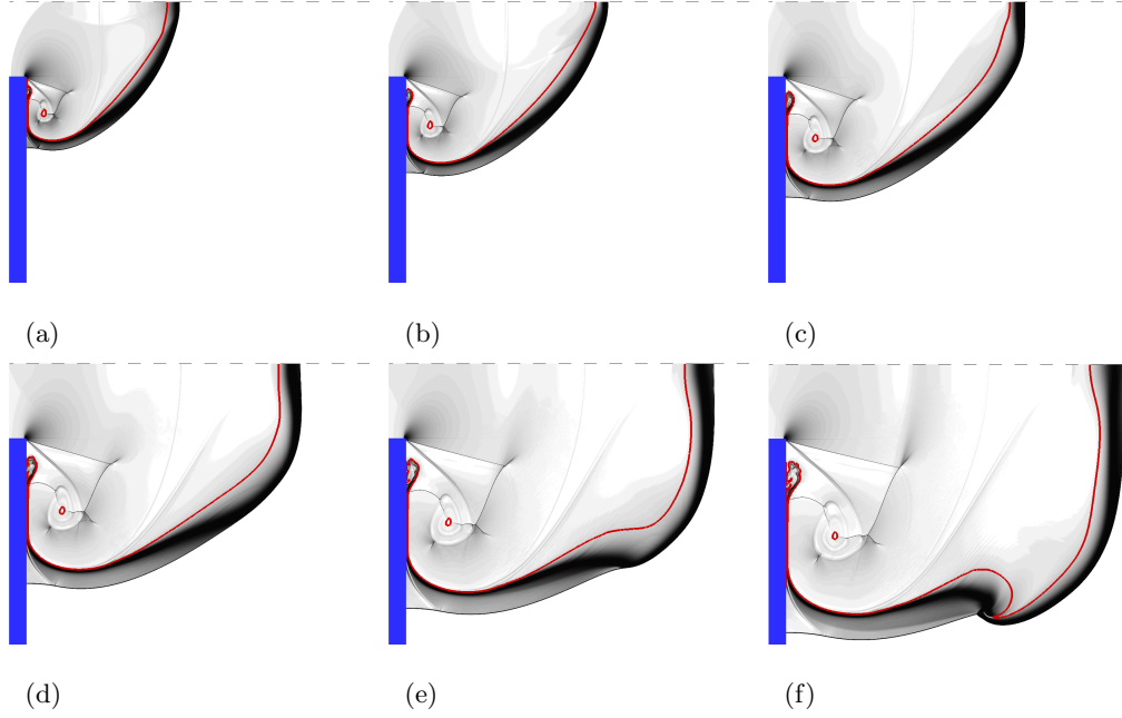
FIGURE 15. Numerical schlieren images for the case \theta_{CJ} = 3.5 . (a) t = 10.17 ; (b) t = 13.83 ; (c) t = 17.49 ; (d) t = 21.15 . (e) t = 24.81 ; (f) t = 28.47 . The solid line is the locus of 95% product.
