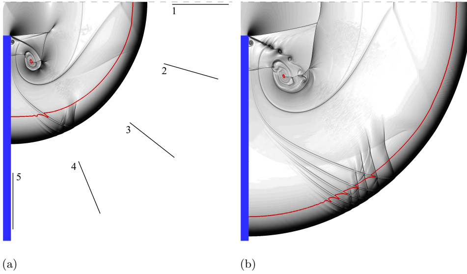
FIGURE 7. Numerical schlieren images for the case \theta_{CJ} = 1 . (a) t = 21.15 ; (b) t = 35.79 . The solid line is the locus of 95% product.
