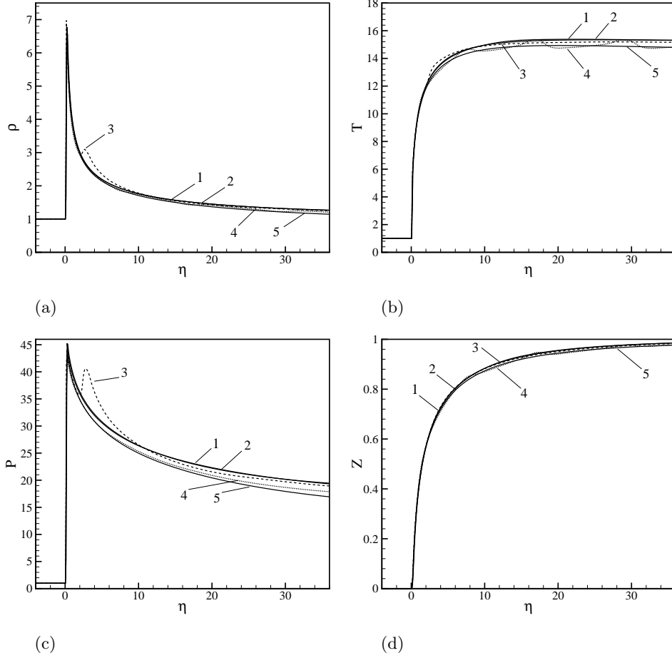
FIGURE 8. Density (a), temperature (b), pressure (c) and progress variable (d) profiles for 5 data sets extracted at t = 35.79 . Slice 1 and 5 are extracted along the plane of symmetry and the corner wall, respectively. The remaining data are taken in the shock normal direction and are evenly spaced along the detonation front.
