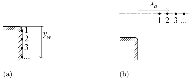
FIGURE 9. Initial location of injected particles along the corner wall (a) and the plane of symmetry (b).
