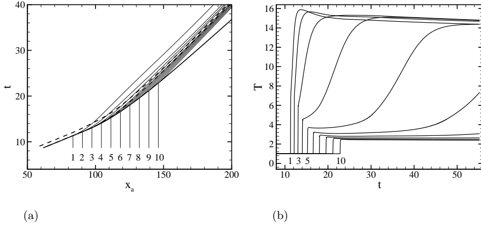
FIGURE 13. Frame (a): particle paths for ten sample particles on the plane of symmetry. Shock (thick solid line); traces of 5% and 95% of reaction completion (dashed lines); particle paths (thin solid lines). Frame (b): temperature profiles along the particles paths.
