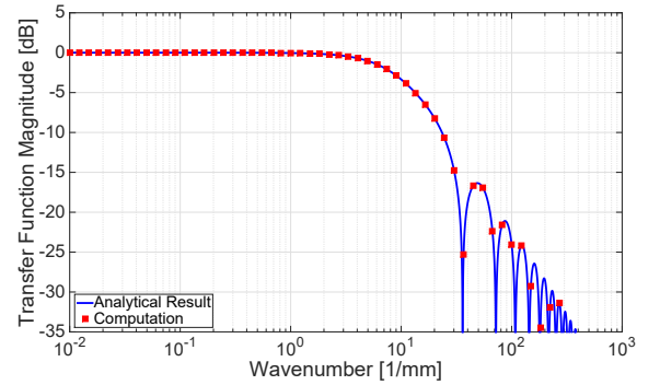
Fig. 10. Transfer function H(k) for the two-beam FLDI for uniform 2-D sinusoidal disturbances in x between z = \pm 10 mm centered at z = 0 .
