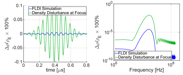
(a) Output of the FLDI simulation for case 4 in Table 5 scaled with the same value of Z found in case 1 compared to the actual density disturbance at the focus.
