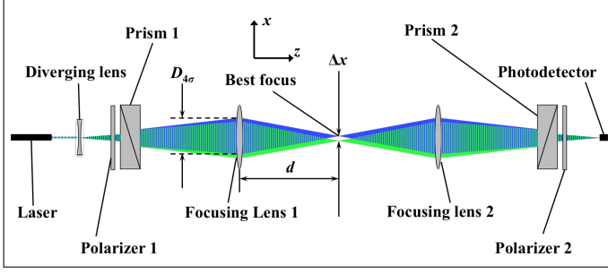
Fig. 1. Schematic of an FLDI setup. The two beams are shown as blue and green. Regions where the beams overlap are shown as striped. The coordinate system shown will be the one used throughout this paper.
