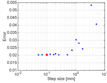
Fig. 12. Convergence study for the transfer function shown in Figure 11. The red square indicates the chosen resolution.
