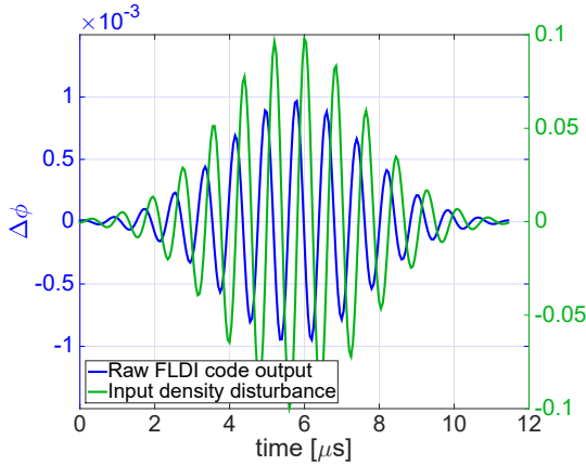
Fig. 21. Output of the FLDI simulation compared to the input boundary layer wave packet density disturbance. The y -axis on the left corresponds to the FLDI output and the y -axis on the right corresponds to the input density at the location of the beams at z = 0 .
