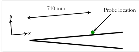
Fig. 19. Cone model used in T5 studies
