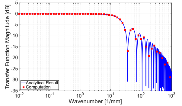
Fig. 9. Transfer function H(k) for the two-beam FLDI for 1-D sinusoidal disturbances in x in an infinitesimally-thin plane at z = 0 .
