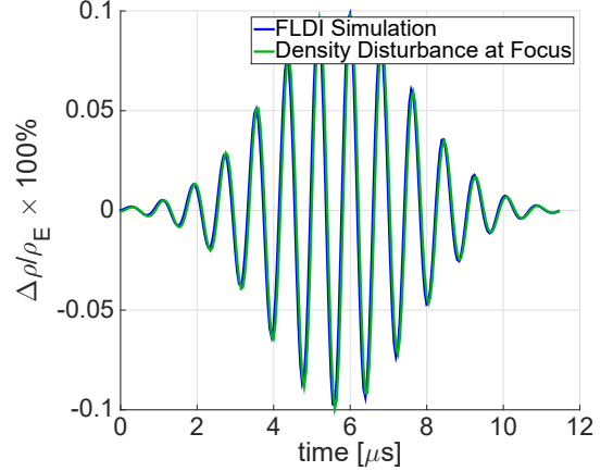
Fig. 22. Output of the FLDI simulation, scaled with Equation 27, compared to the input boundary layer wave packet for the optimum value of Z = 12.6 mm.
