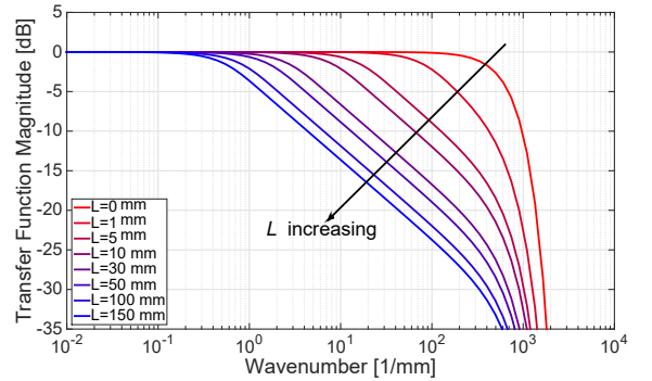
Fig. 6. Transfer function of Equation 16 plotted for various values of L . As L increases, or, as more signal away from best focus is considered, the error function in Equation 16 contributes a k^{-1} rolloff beginning at lower values of k . This leads to attenuation of high-wavenumber disturbances away from best focus.
