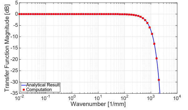
Fig. 5. Transfer function H_w(k) for a single beam for 1-D sinusoidal disturbances in x in an infinitesimally-thin plane at z = 0
