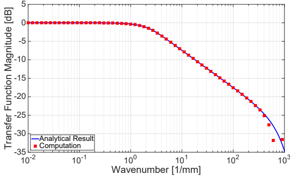
Fig. 8. Transfer function H_w(k) for a single beam for uniform 2-D sinusoidal disturbances in x between z = \pm 30 mm centered at z = 0 .
