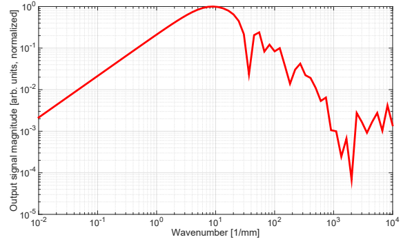
Fig. 13. Normalized FLDI output signal for sinusoidal disturbances within \pm 10 mm of the focus in z , corresponding to the transfer function plotted in Figure 10.
