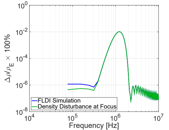
Fig. 23. PSD of the FLDI simulation, scaled with Equation 27 and optimum Z value, compared to the PSD of the input boundary layer wave packet.
