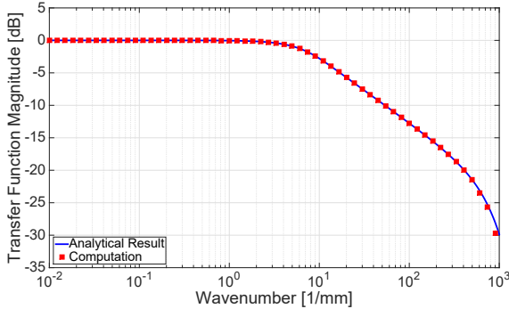
Fig. 7. Transfer function H_w(k) for a single beam for uniform 2-D sinusoidal disturbances in x between z = \pm 10 mm centered at z = 0 .
