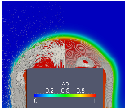
Fig. 16. Steady-state result of OpenFOAM computation of the flow out of the argon jet. Velocity vectors are shown on the left and streamlines on the right. Both are superimposed on a contour plot of argon mass fraction. L_{\text{jet}} is the length out of the page (in z ) that the cross-section shown here extends.
