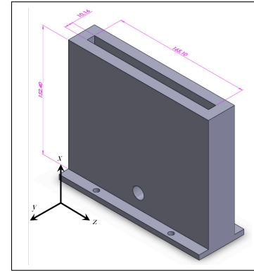
Fig. 14. A solid model of the chamber for the argon jet with dimensions given in mm. The coordinate system shown corresponds to the orientation of the coordinate system of the FLDI beams.
